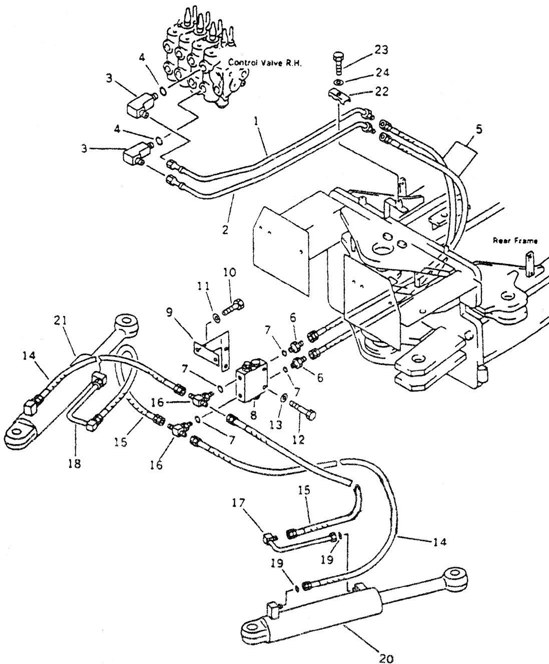
FIG. 6423A 液压管路(铰接控制管路) HYDRAULIC PIPING (ARTICULATE CYLINDER LINE)
