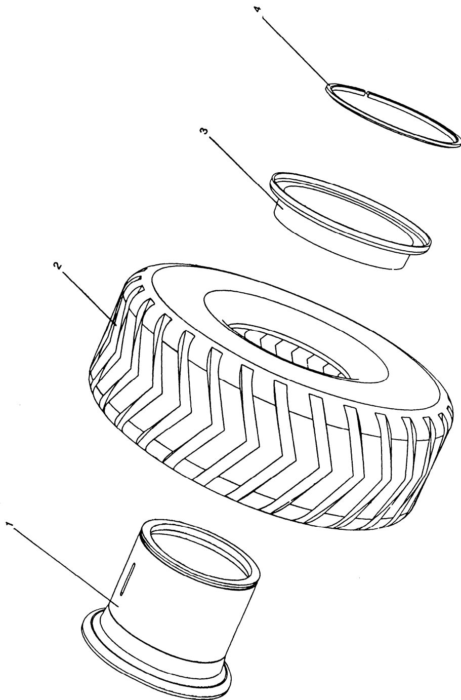
FIG. 3001 轮胎和轮辋 WHEEL AND TUBELESS TIRE
