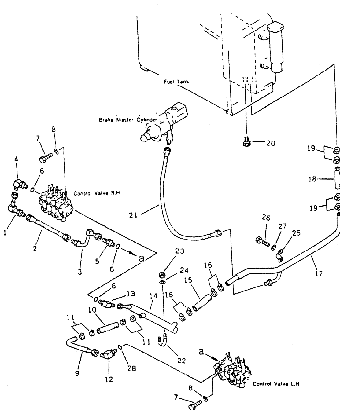
FIG. 6403 液压管路(多路阀至油箱) HYDRAULIC PIPING (CONTROL VALVE TO TANK)
