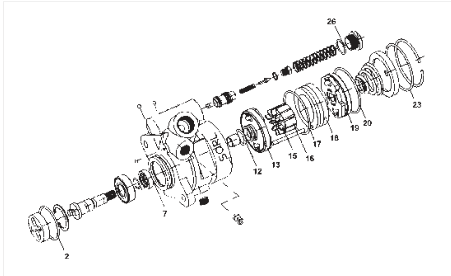
STEERING PUMP (CHINA)
