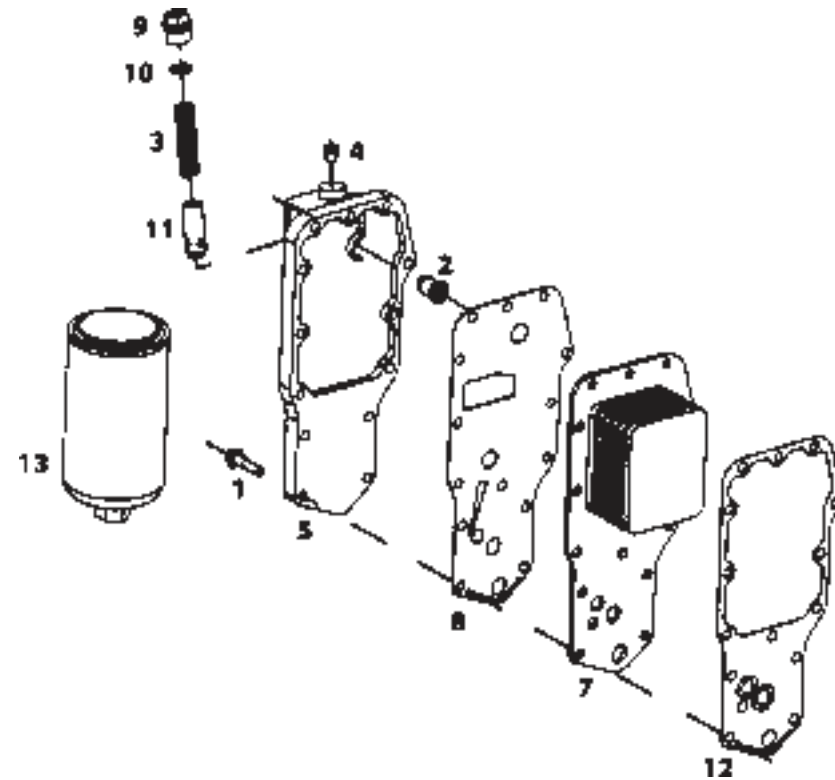
LUBRICATING OIL COOLER/OIL FILTER
