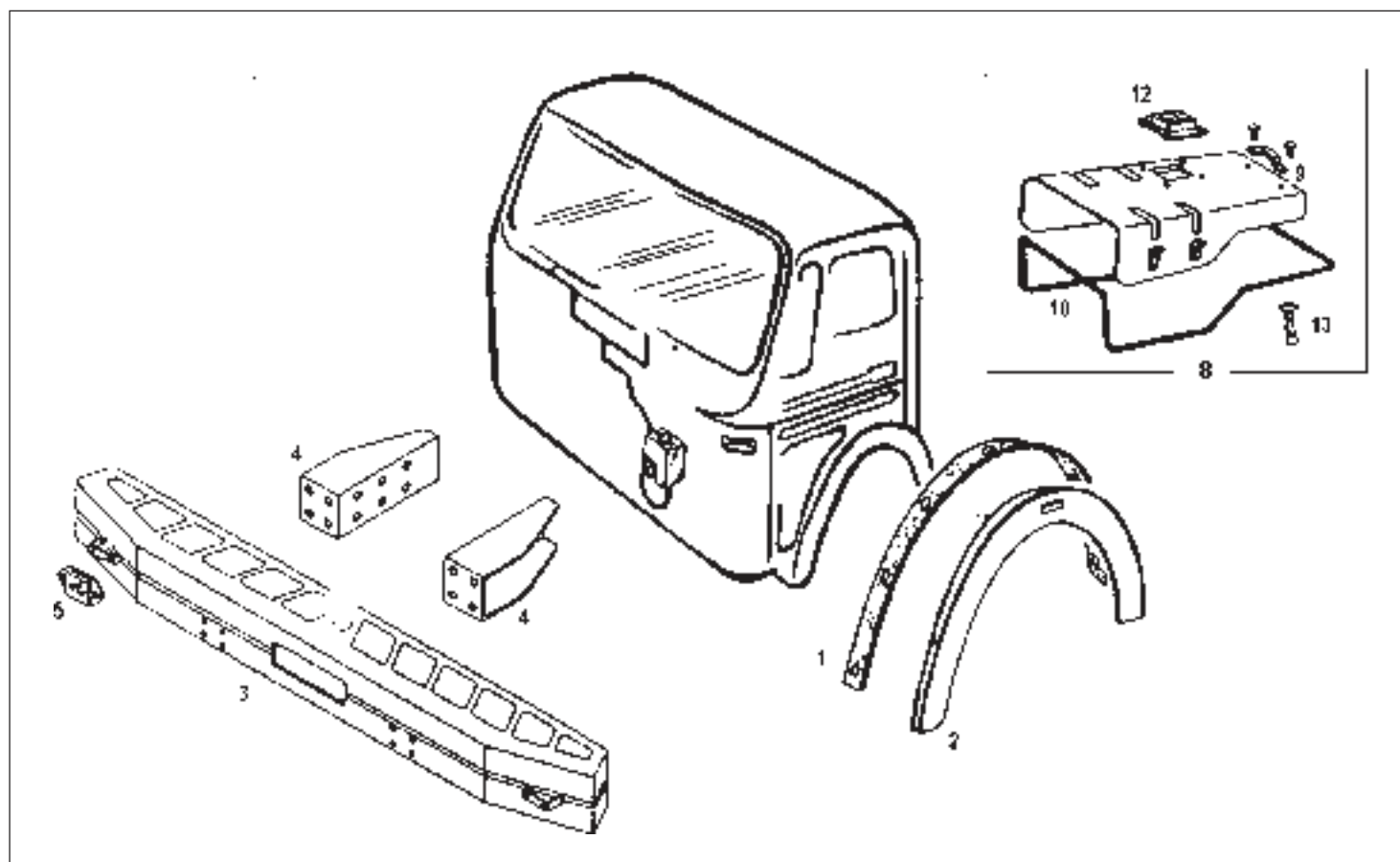
BUMPER, ENGINE HOOD, FENDER
