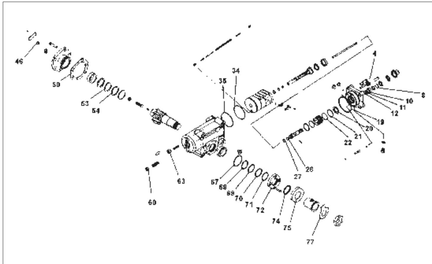
STEERING GEAR BOX (CHINA)
