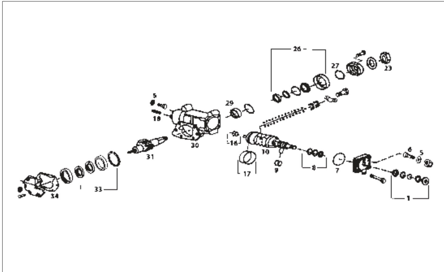
STEERING GEAR BOX (RANE)
