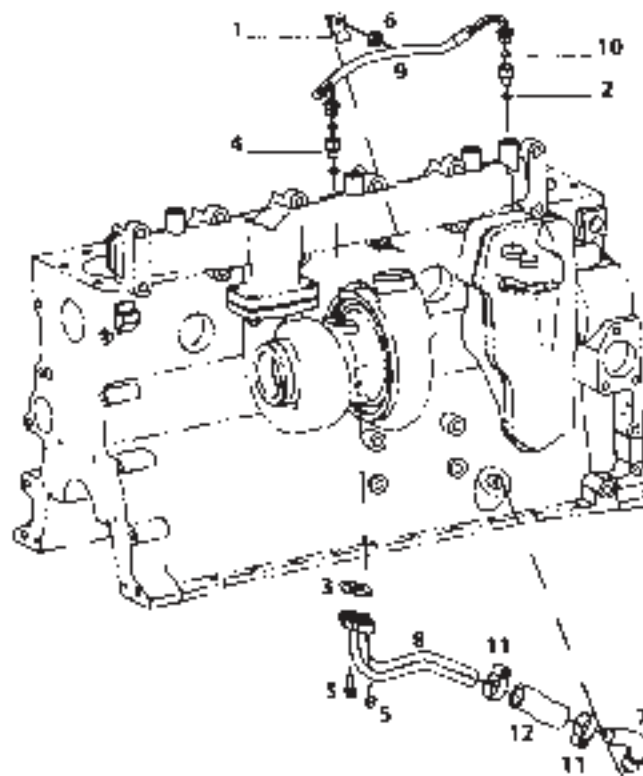
TURBOCHARGER PLUMBING
