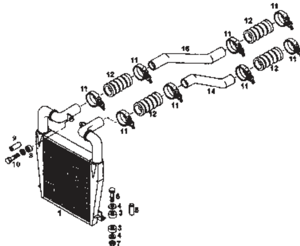
INTERCOOLER AND INTERCOOLER CONNECTION
