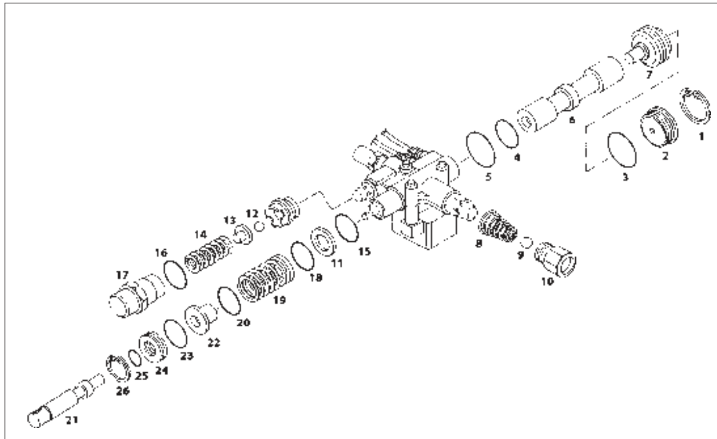
TIPPING VALVE (3 DHMP)
