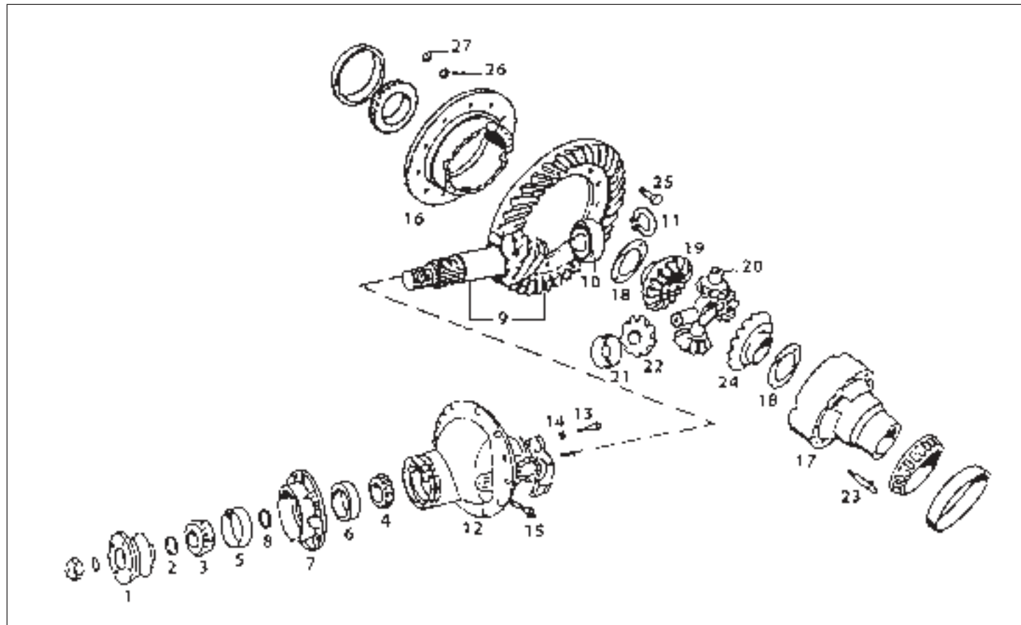
REAR, REAR CARRIER (INTER AXLE)
