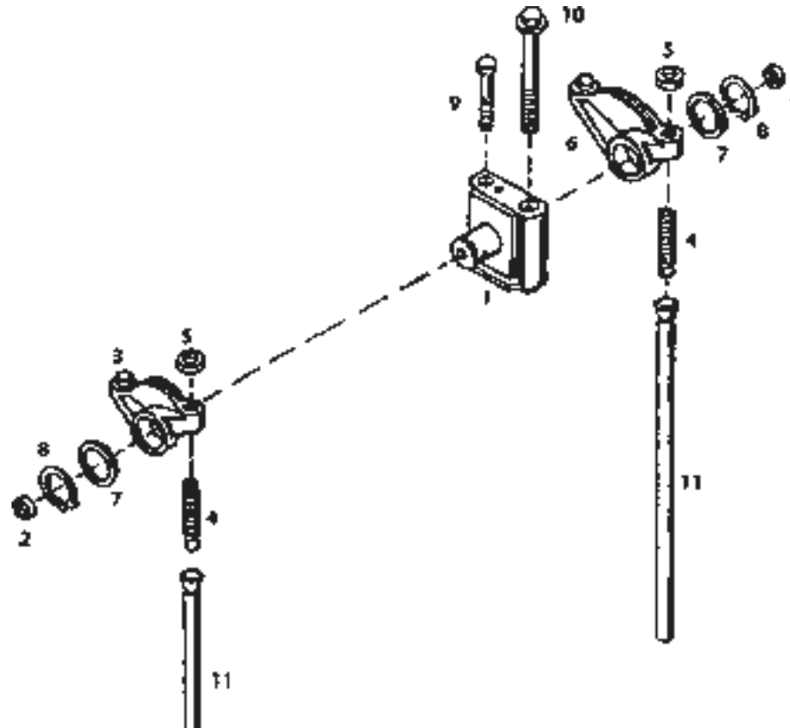
ROCKER LEVER
