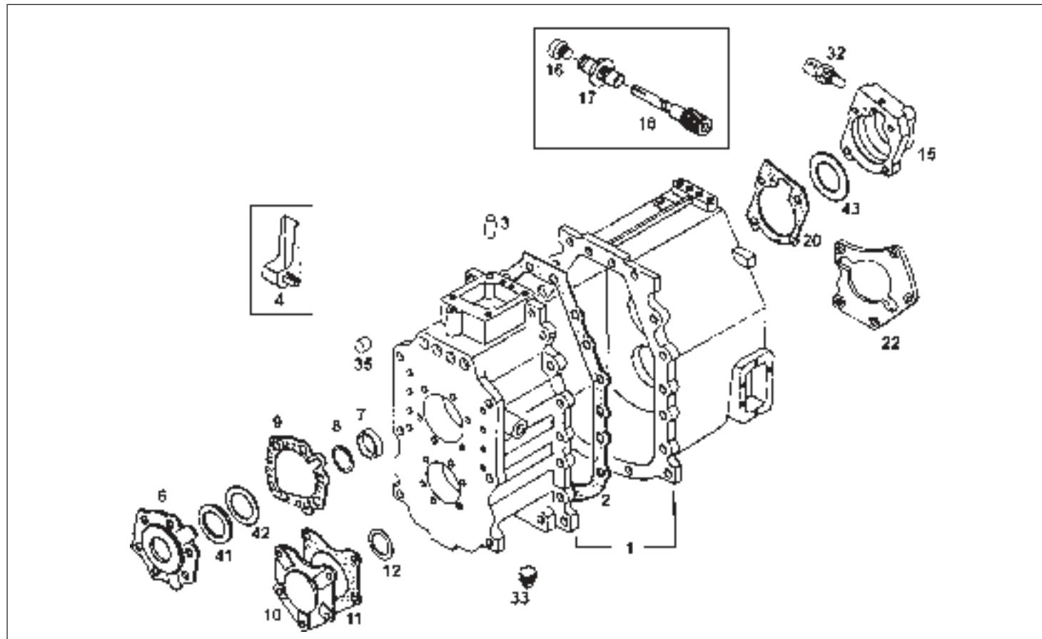
GEAR BOX, HOUSING AND COVERS (G 600)
