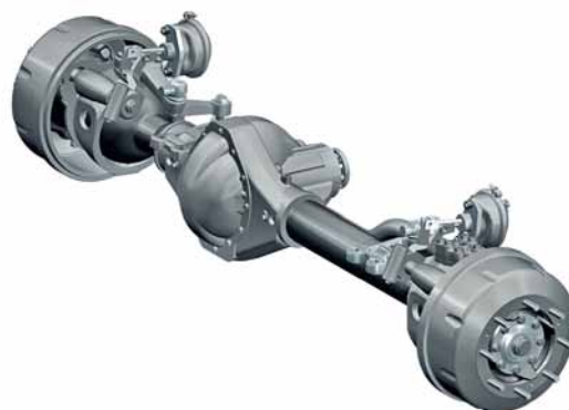
Front axle, 6,0 t (731.721)
