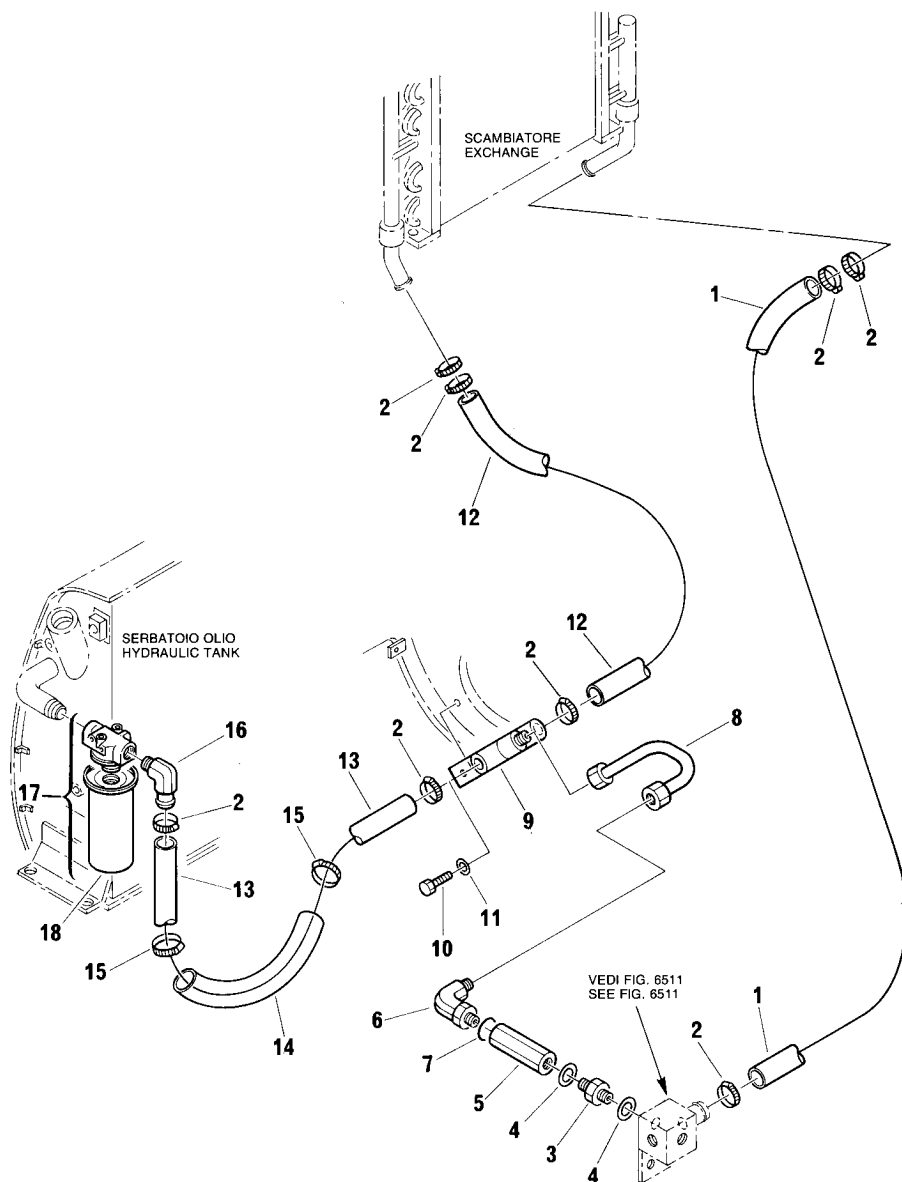
FIG. 6516 IMPIANTO IDRAULICO SCARICO (2/2) HYDRAULIC PIPING (RETURN LINE) (2/2)
