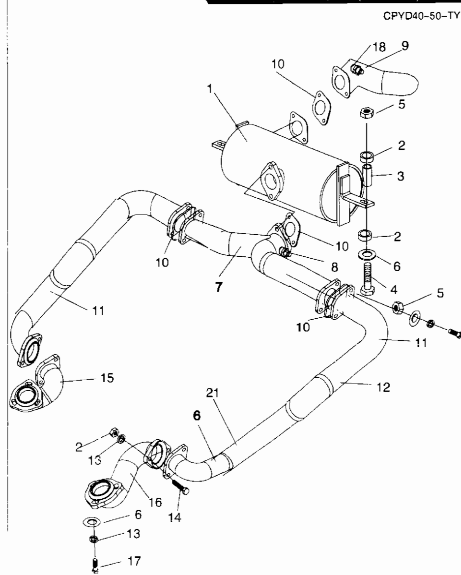
排气系统(液化气机)/EXHAUST SYSTEM(LPG)
