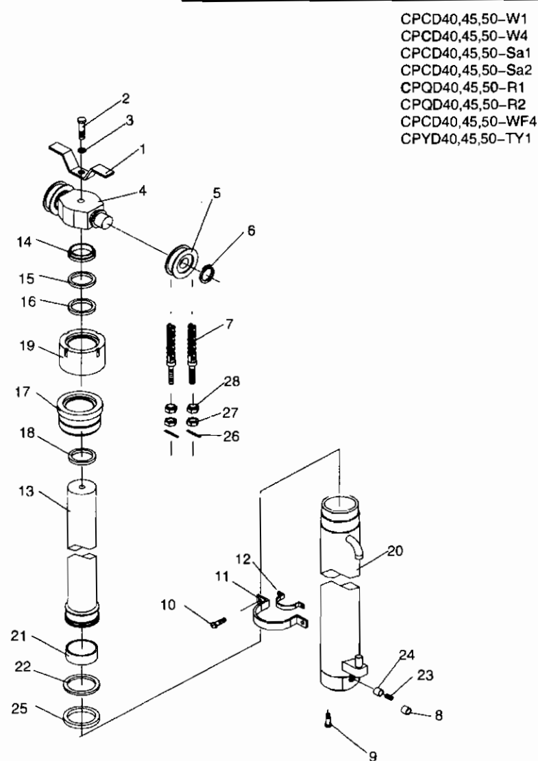
前起升油缸(三级全自由)/FRONT LIFT CYLINDER(WIDE VIEW FULL FREE 3-STAGE MAST KZSM) 图79/FIG79
