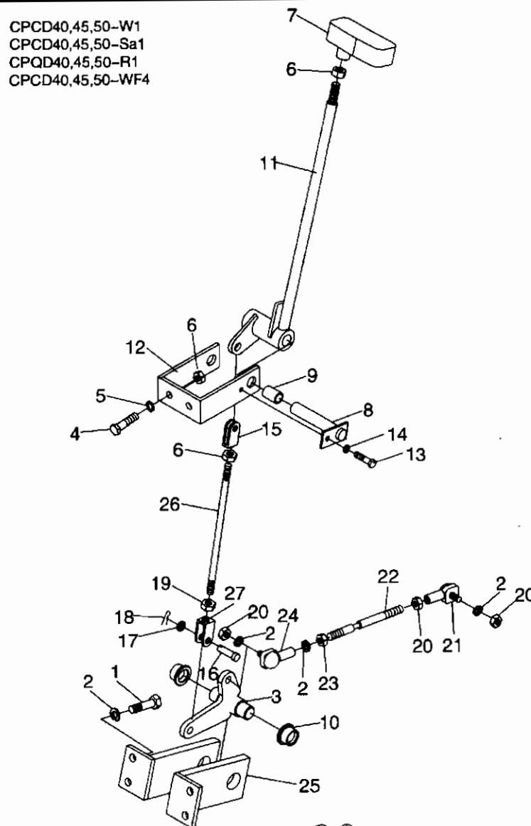
变速箱变速操纵/TRANSMISSION CONTROL LINKAGE
