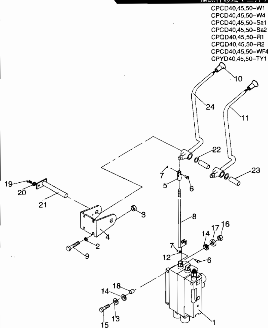
操纵杆总成 (二片) / VALVE CONTROL LINKAGE ( TWO-THROW )
