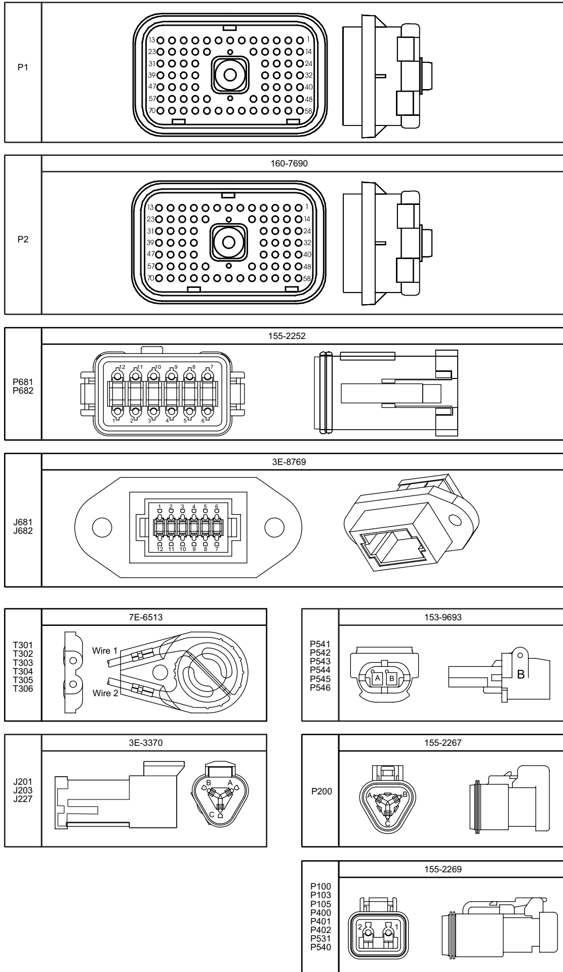
Connector Tables for Harness 241-3150 -01
