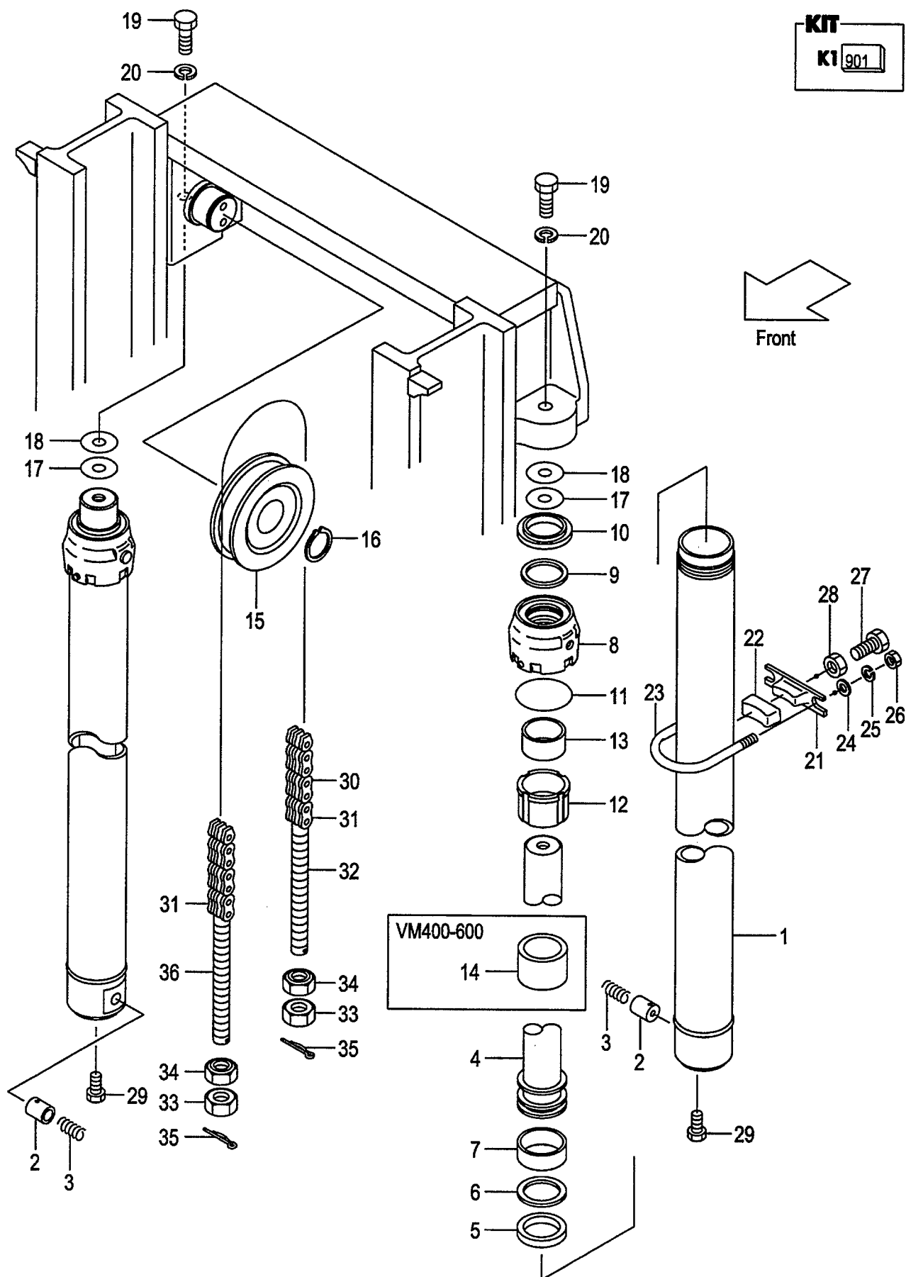
FIG.94 LIFT CYLINDER [VM43A] (M6048410) リフトシリンダ
