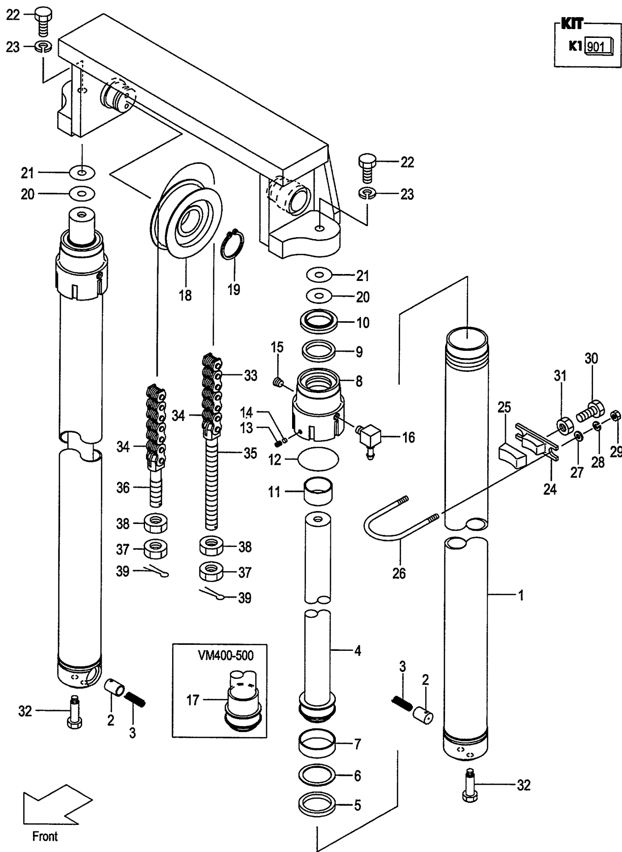
FIG.106 LIFT CYLINDER [VM43H] (M6048450) リフトシリンダ
