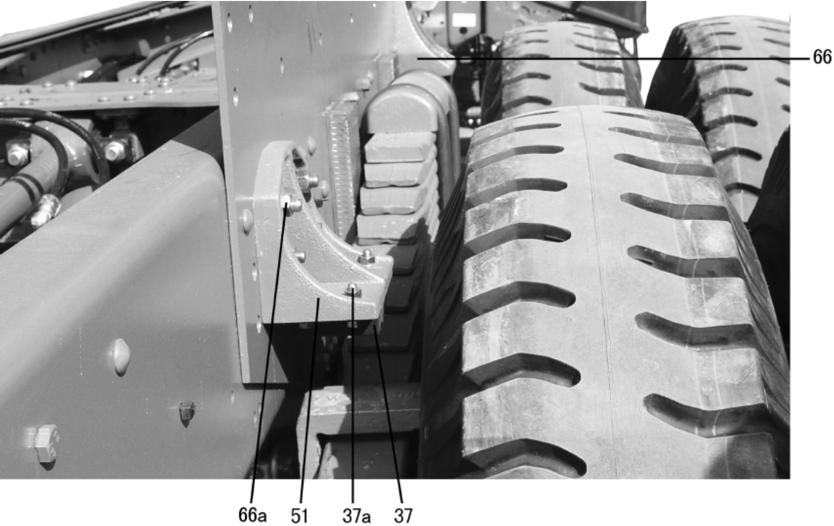
C8-4 6×4, 8×4 SWIVEL SPRING AND SUSPENSION/6×4, 8×4平衡悬架
