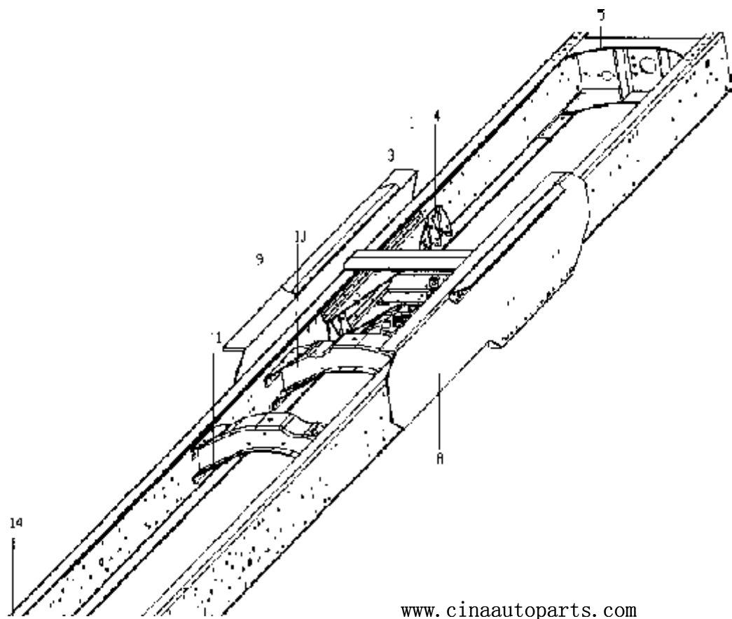
C7-5 CHASSIS FRAME FOR 6×4 TRACTOR TRUCK/6×4牵引车车架
