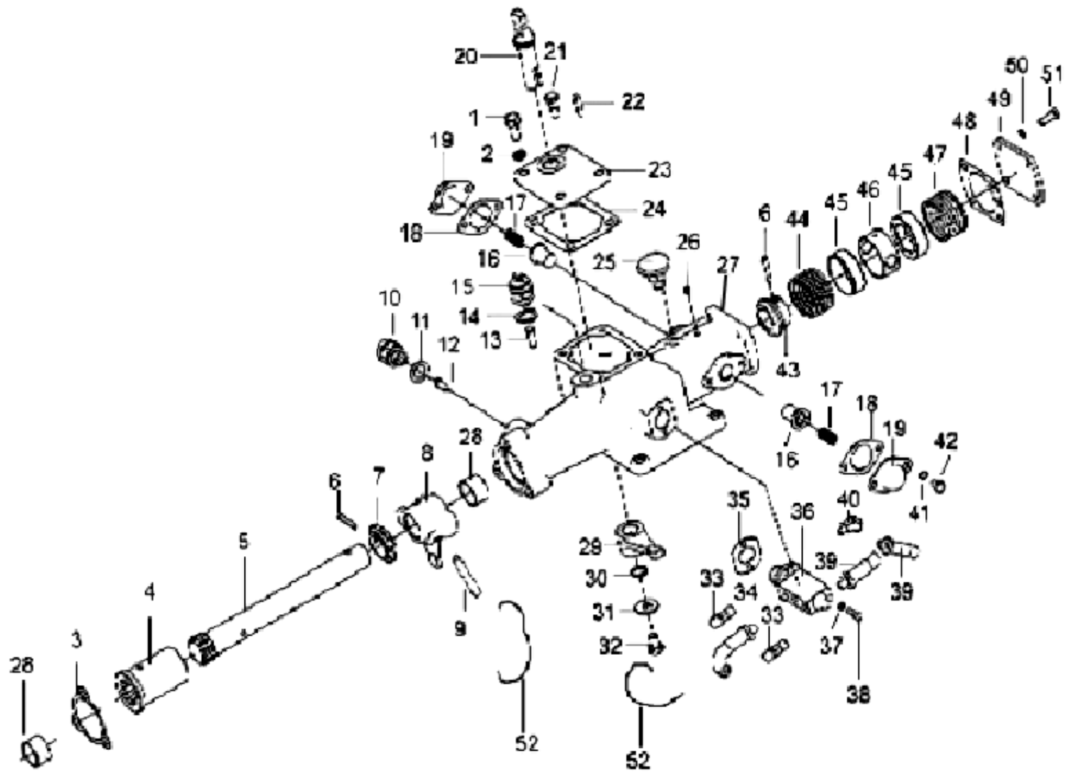
C4-7 9JS150T DOUBLE H OPERATION/双H换档控制机构
