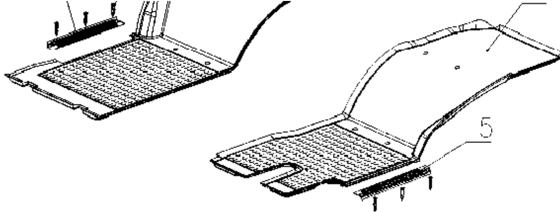
C12-7 ENGINE HOOD, FLOOR LINING FOR STANDARD CAB/标准驾驶室发动机罩、地板
